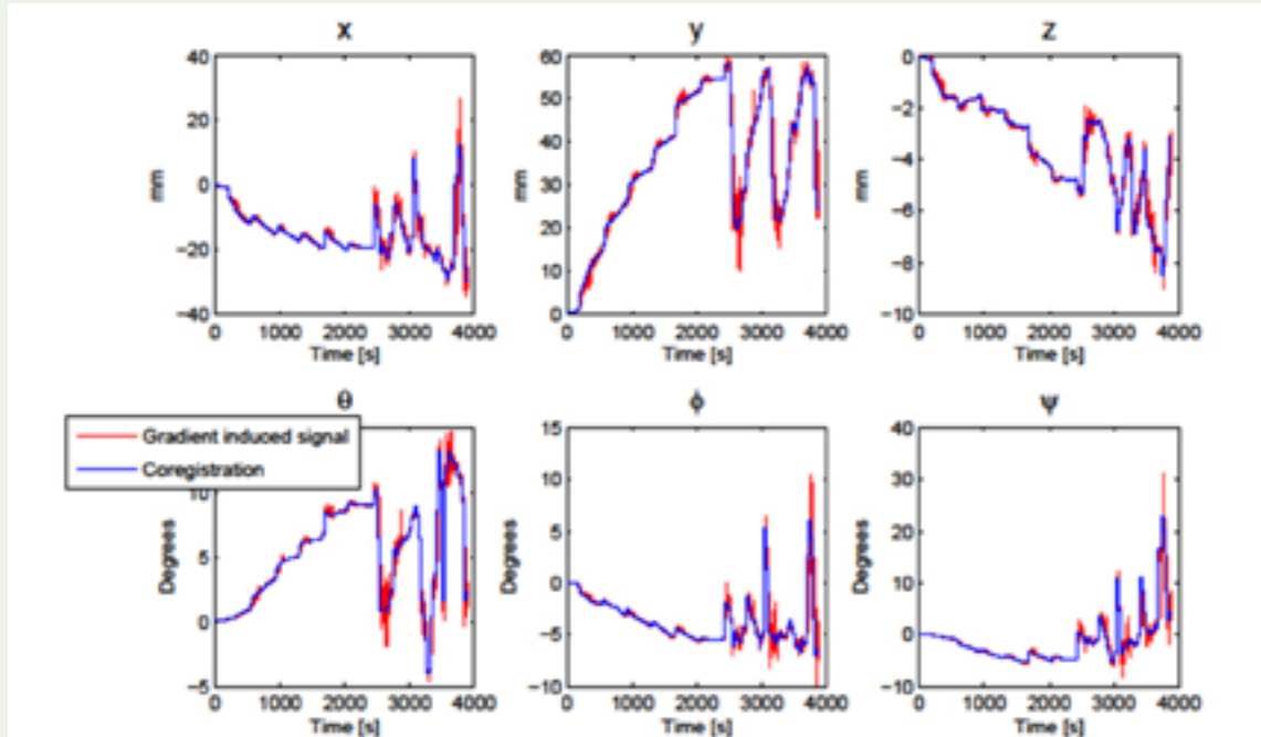
Figure 1: In the MSc project by Mark B. Vestergaard it was shown that patient motion can be tracked during MRI using EEG equipment. The method was subsequently improved regarding accuracy and temporal resolution. The curves show the evolution of parameters characterizing person motion during a 4000 second scan. Using inflatable pillows, the head is moved in a semi-controlled way during the first half of the scan, and is moved freely by the scanned person thereafter. Parameters extracted from the EEG (red) correlate well with parameters extracted from MRI (blue) but the prior can be acquired more rapidly, and be used to improve MRI. When the high frequency noise apparent in the EEG data is filtered, motion tracking with sub-millimeter precision results.
