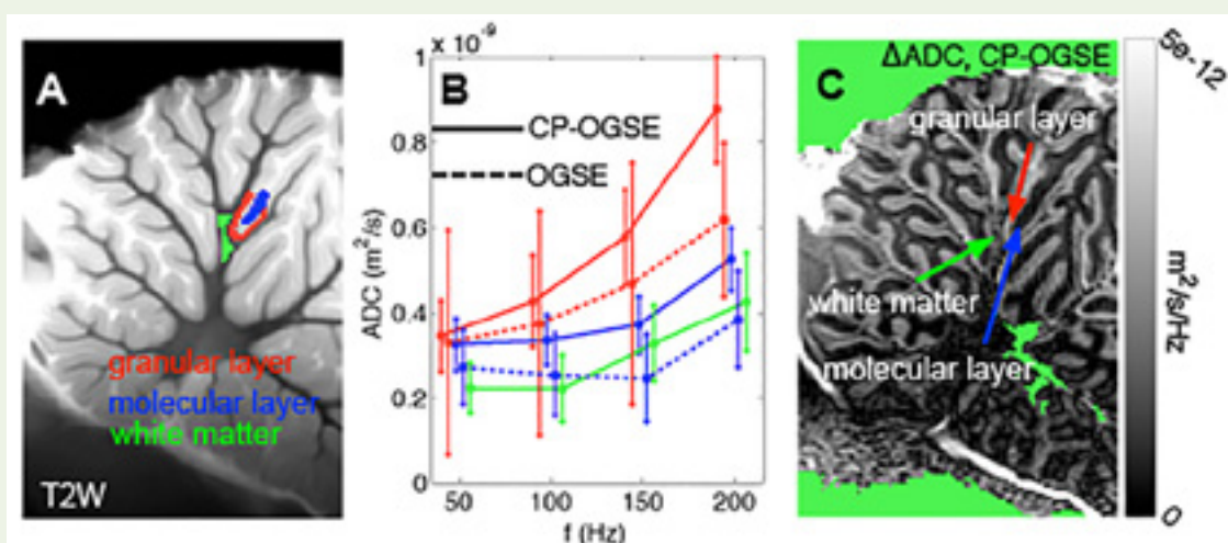
Figure 2: Oscillating gradient spin echo (OGSE) can capture diffusion processes on much shorter times scales than conventional diffusion weighted imaging and provides a new contrast to tissue microstructure. A) shows a T2-weighted image of the monkey cerebellum with three regions of interest covering different tissue types. The granular and molecular layers are not distinguishable in conventional modalities, but the tissues are well separated at high OGSE frequencies (red and purple solid lines in B). This contrast mechanism can be used to create new maps corresponding to cellular density as shown in figure C).
