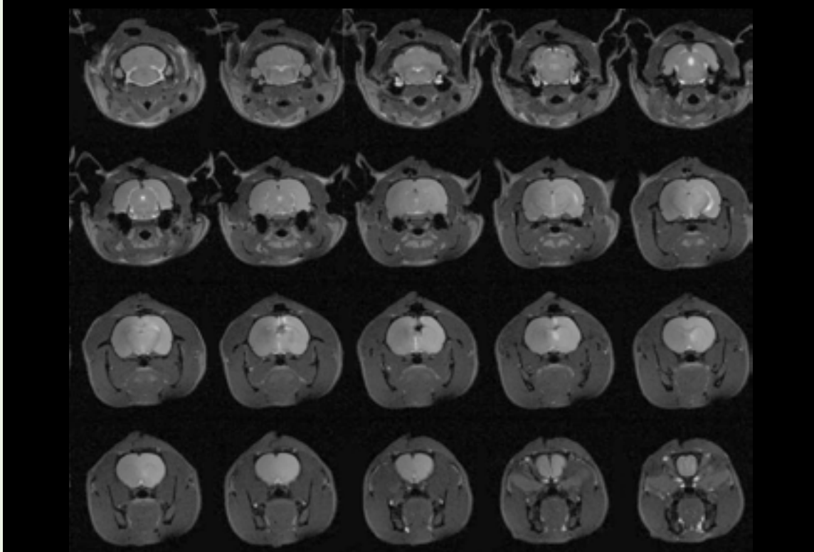
Figure 1: T1-weighted imaging one day post implantation of osmotic micropump catheter in right hemisphere of a normal rat brain. In vivo imaging after 24h of Gadolinium infusion revealed contrast enhancement in the ipsilateral part of the ventricular system including third ventricle. In addition contrast enhancement was seen in whole of the ipsilateral hemisphere. This confirmed the use of the osmotic micropumps for intracerebroventricular drug administration.
