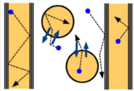
Figure 1: Schematic view of water exchange across the cell membranes of permeable gliacells and impermeable nerve fibers. Water exchange across the cell membrane is an important regulatory mechanism and alterations of the cell membrane permeability are associated with diseases such as cancer and Parkinson's disease. The DIG group is actively developing and implementing novel methods to provide clinically feasible in vivo measurements of the membrane permeability using non-invasive MR technology.
