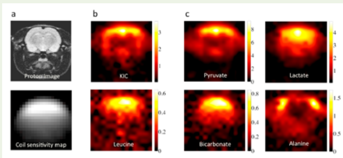
Figure 1: Chemical shift imaging of rat brain BCAT activity in vivo . a) Anatomical proton image and the surface coil sensitivity profile are shown. b) Metabolic maps of [1-^{13}\text{C}] KIC and [1-^{13}\text{C}] leucine (sum of 6) recorded 20 s after end of hyperpolarized [1-^{13}\text{C}] KIC injection. Hyperpolarized [1-^{13}\text{C}] leucine is specifically observed inside the brain. c) Hyperpolarized [1-^{13}\text{C}] pyruvate was used as a reference substrate and its metabolic map is shown together with [1-^{13}\text{C}] lactate, [1-^{13}\text{C}] bicarbonate and [1-^{13}\text{C}] alanine (sum of 6). Absolute color scale is shown for each metabolite image (a.u.).
