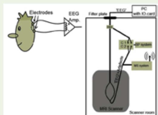
Figure 2: The EEG-fMRI validation setup developed for Mads Andersen's MSc project. A normal pre-recorded EEG synthesized by a PC is sent through the scanner and mixed with scanner-induced noise. Both the noisy and the noise-free signals are sampled in a traditional MR-compatible EEG system ("BP system"). For comparison, the signals were also measured with a home-built EEG system ("MS system"). The systems were compared, and algorithms for removing scanner noise validated by comparing noise-free and noise-corrected signals.
