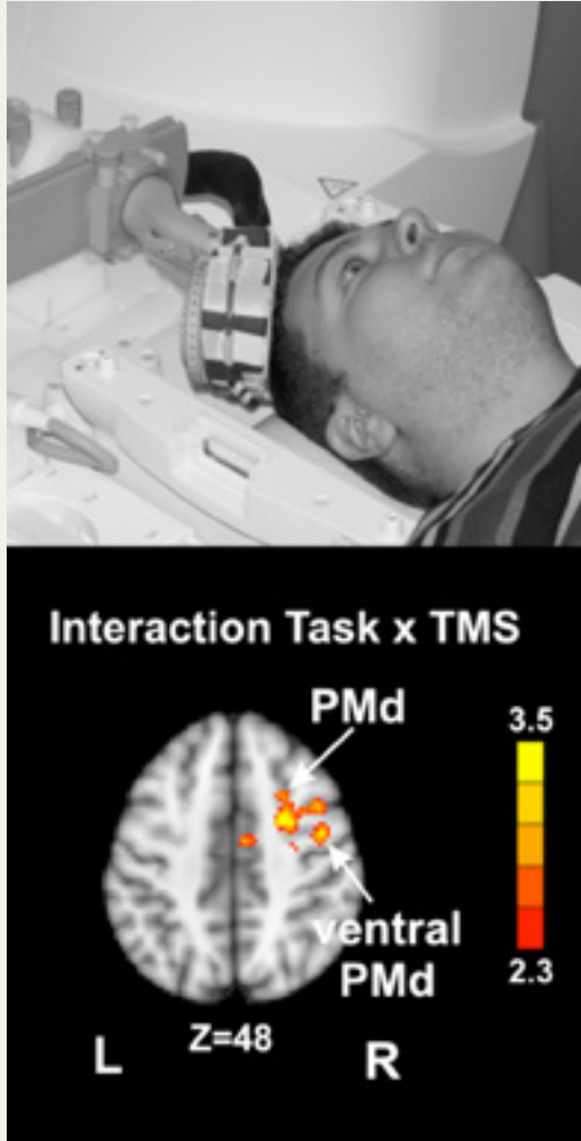
Figure 3: Top: Setup for interleaved TMS-fMRI. Bottom: The interaction between task and TMS effects demonstrates that the remote effects of left PMd stimulation depend on the behavioral task
