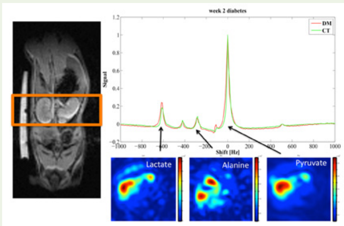
Figure 2: Kidney metabolism of intravenously injected hyperpolarized [1-^{13}\text{C}] pyruvate. Axial metabolite maps (lower right) of lactate, alanine and pyruvate from a healthy rat are shown together with averaged spectra (upper right) corresponding to the sum of all kidney pixels for a group of diabetic rats (red curve) and a group of control animals (green curve). The position of the axial slice is indicated on the proton image (left).
